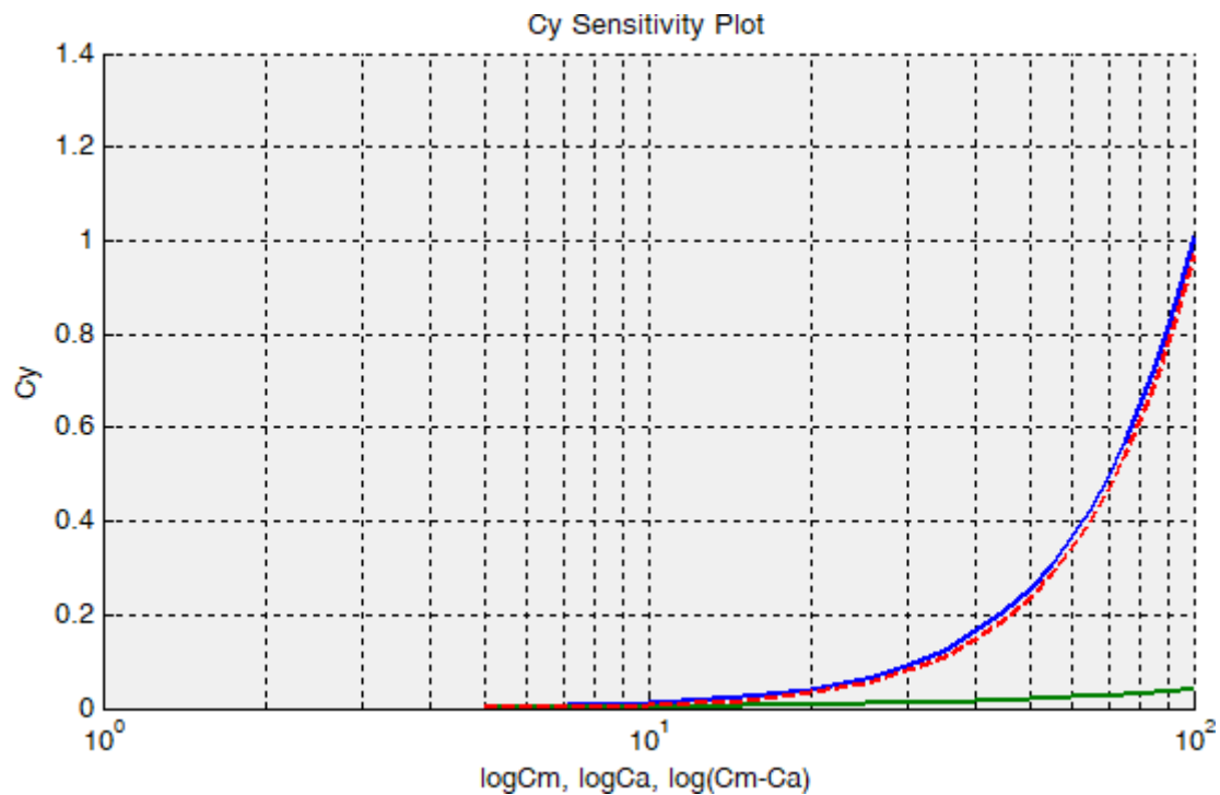
Figure 3. c_y = f(\log c_m, \log c_a)
