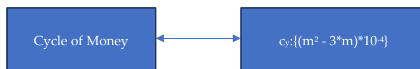
Figure 1. Cycle of money for c_y: \{(m^2 - 3^* m) * 10^{-4}\}
